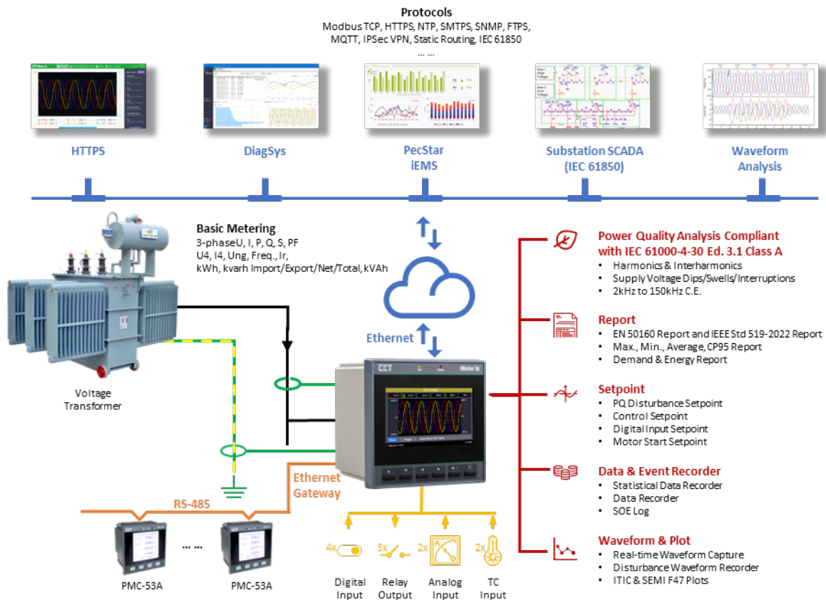
Figure 1-1 Typical Application
