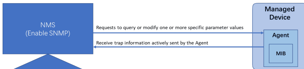
Figure 4-47 SNMP Structure
