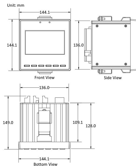
Figure 2-2 Unit Dimension
