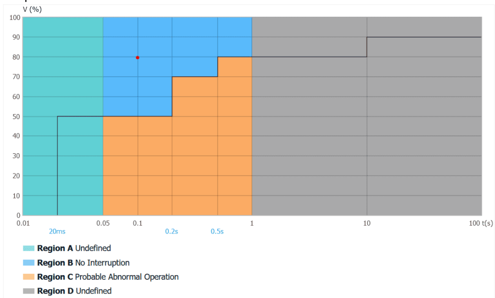
Figure 4-19 SEMI F47 Plot Descriptions
