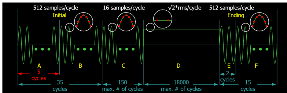
Figure 4-28 DWR Stages
