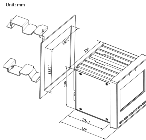
Figure 2-3 Installation
