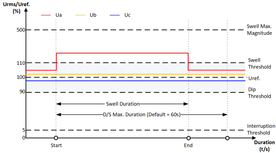
Figure 4-2 Swell Detection Criteria
