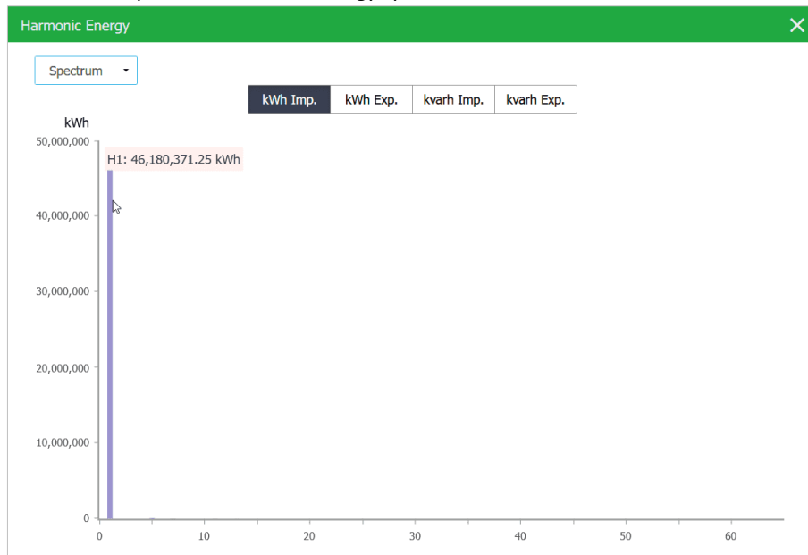
Figure 3-72 Individual Harmonics Spectrum
