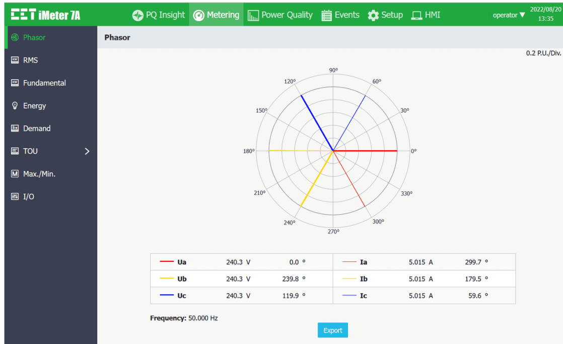
Figure 3-68 Phasor Diagram
