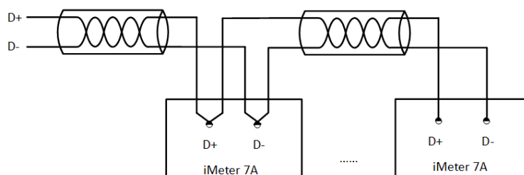
Figure 2-11 RS-485 Communication Connections
