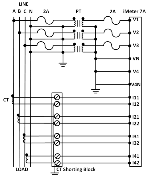
Figure 2-5 3-Phase 4-Wire Wye with 3PTs and 4CTs
