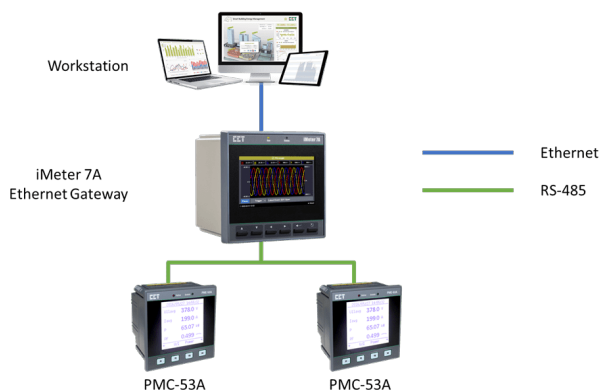
Figure 4-46 Typical Application for Ethernet Gateway
