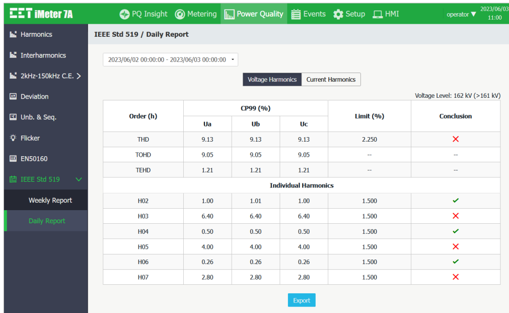
Figure 3-106 IEEE Std 519 Voltage Harmonics Compliance Daily Report
