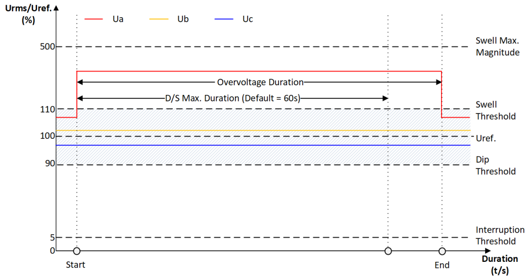
Figure 4-4 Overvoltage Detection Criteria 2
