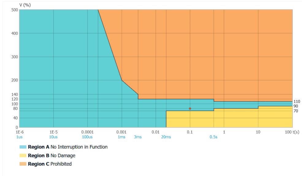
Figure 4-18 ITIC Plot Descriptions
