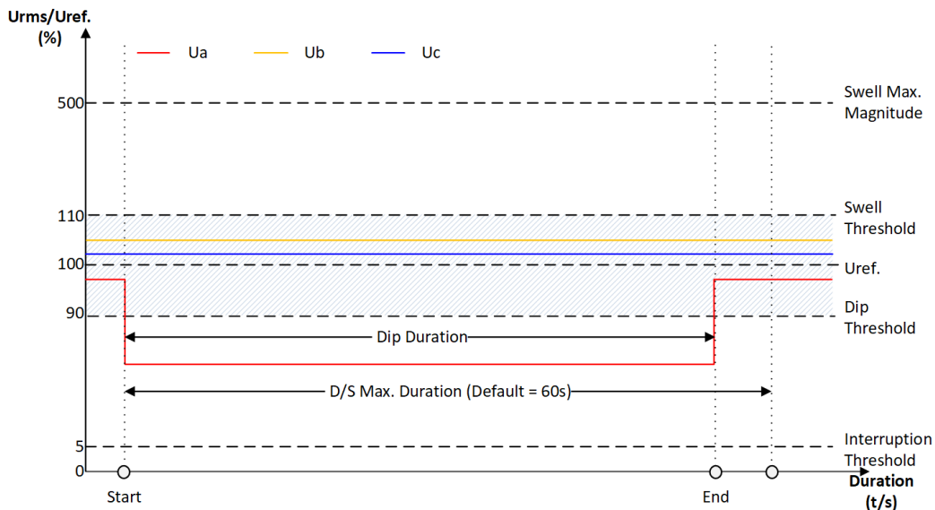
Figure 4-5 Dip Detection Criteria
