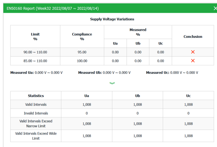
Figure 3-93 Supply Voltage Variations
