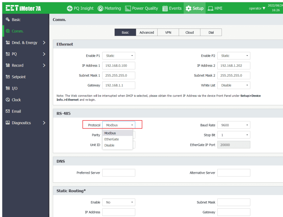
Figure 4-45 Select "EtherGate" Mode on the Web Server
