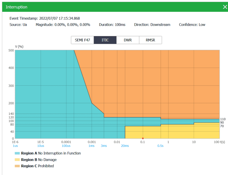
Figure 3-112 Interruption on ITIC Interface
