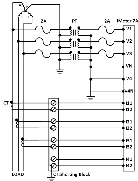
Figure 2-7 3-Phase 3-Wire Grounded Wye with 3PTs & 3CTs
