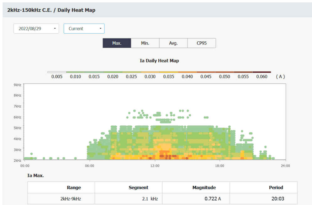
Figure 4-16 Daily Heat Map for Ia Max.
