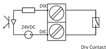
Figure 2-13 DI Connections
