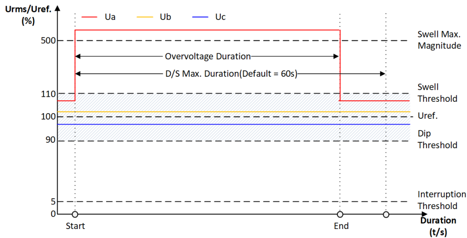
Figure 4-3 Overvoltage Detection Criteria 1
