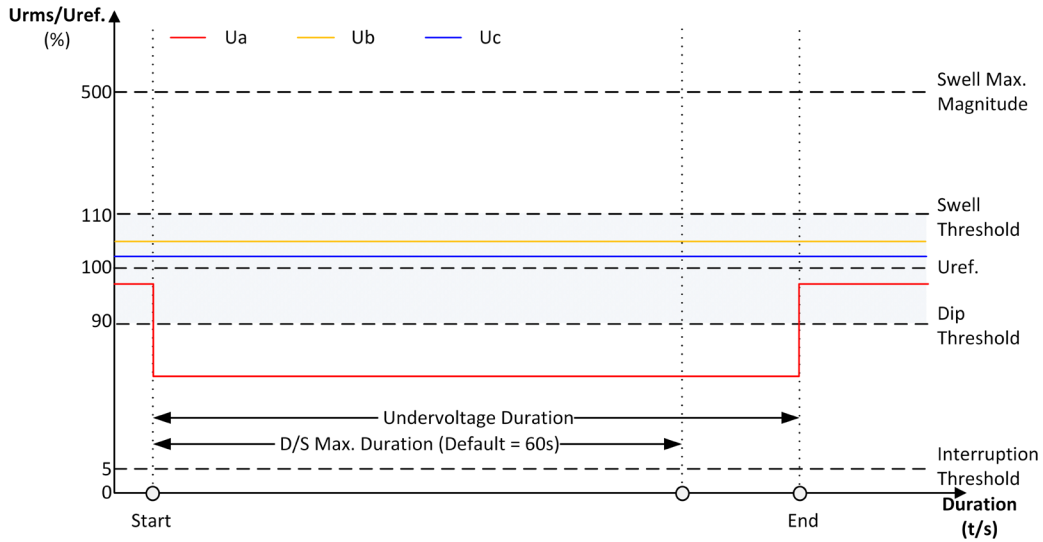
Figure 4-7 Undervoltage Detection Criteria
