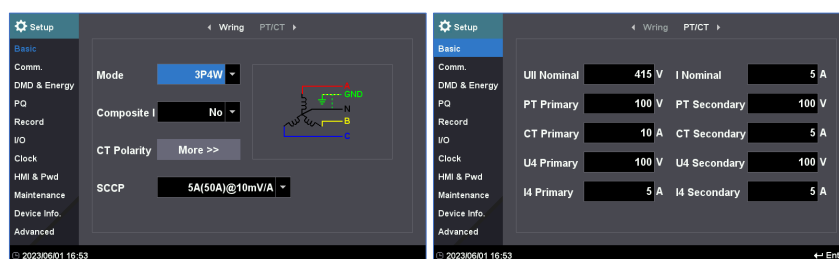
Wiring Setup
