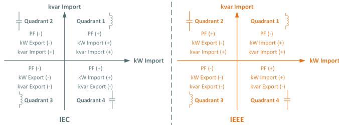
Figure 5-1 PF Convention
