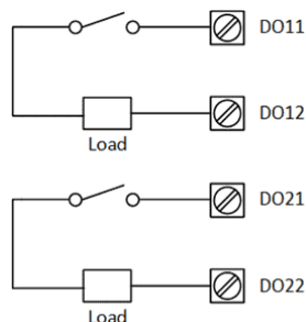
Figure 2-16 DO Connections
