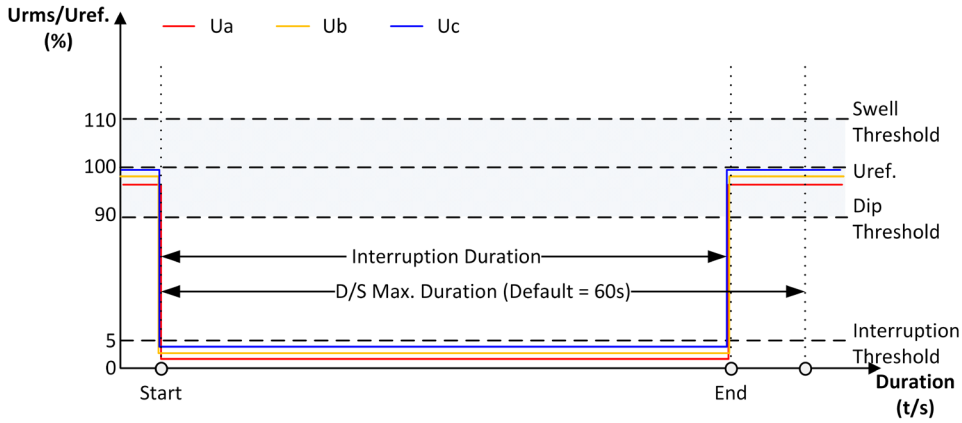
Figure 4-6 Interruption Detection Criteria
